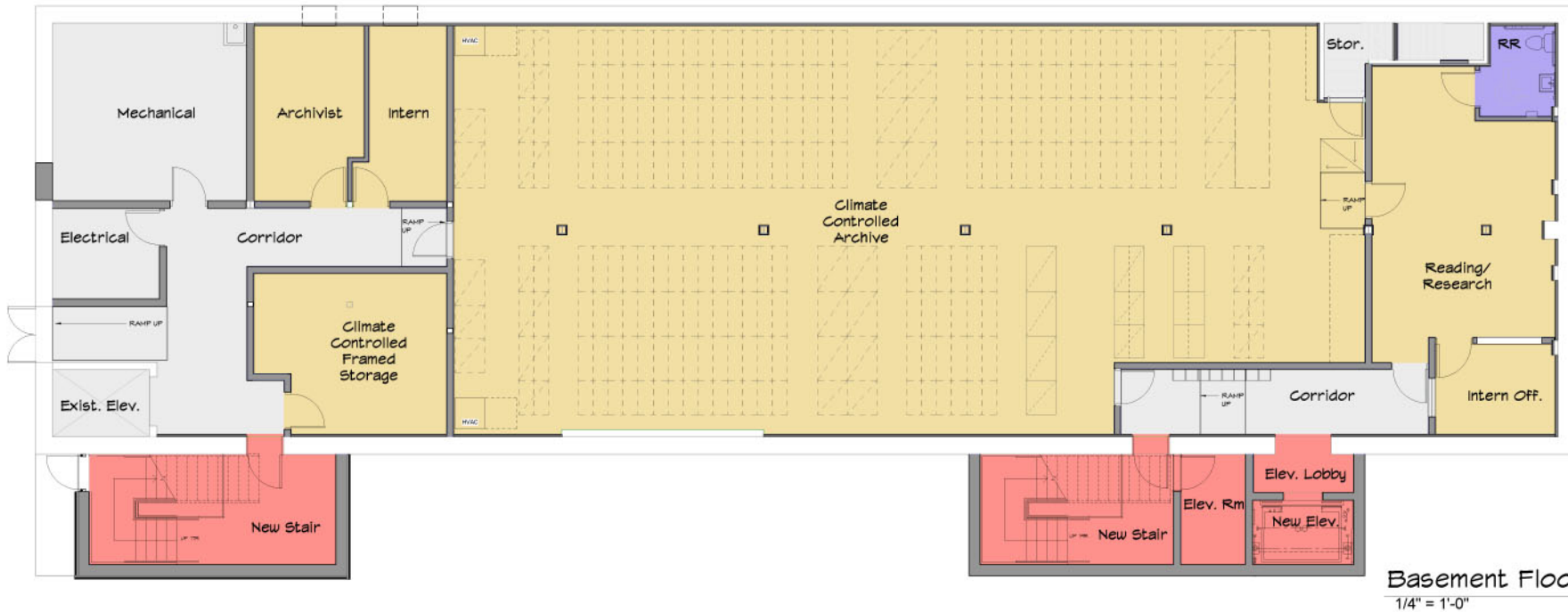
First Floor Plan ⊗ 1/4" = 1'-0"
