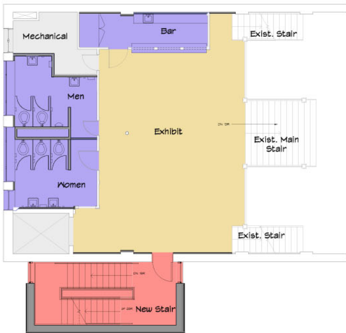
Mezzanine Floor Plan ⊗ 1/4" = 1'-0"
